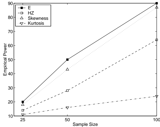
Figure 2: Empirical power of tests of multivariate normality ( d=5 , n=25, 50, 100 ) against normal location mixture .9N_5(0, I) + .1N_5(2, I) : percent of significant tests of 2000 Monte Carlo samples at \alpha = .05 . E denotes the energy test and HZ denotes the Henze-Zirkler test.
