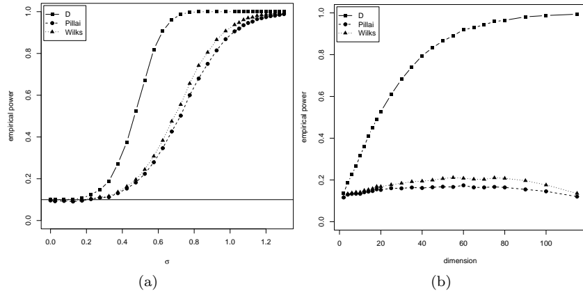
Figure 3: Monte Carlo results for Example 3. Power of the DISCO ( D ) and MANOVA (Wilks, Pillai) tests for Gamma(shape=2, rate=0.1) data, in four groups with n = 30 per group. Group 1 is Gamma(shape=2, rate=0.1) with multiplicative errors distributed as Lognormal( \mu = 0, \sigma ). In (a) dimension p = 10 and \sigma varies and in (b) p varies and \sigma = 0.4 .
