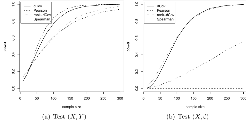
Figure 4: Power comparison of distance covariance and correlation tests at 10% significance level for Gumbel's bivariate exponential distribution. In (a) the null is H : X, Y are independent; (b) tests of independence of X and \varepsilon , where \varepsilon are residuals of the regression of Y on X .
