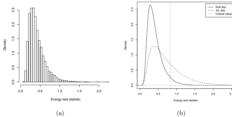
Figure 1: Sampling distribution of the energy goodness-of-fit statistic for univariate normality, sample size n = 30 , in Example 1. Figure (a) displays simulated replicates of the statistic under the null hypothesis. Figure (b) compares the density of n\hat{\mathcal{E}}_n under the null and alternative hypotheses, for a normal location mixture. The rejection region is in the upper tail.
